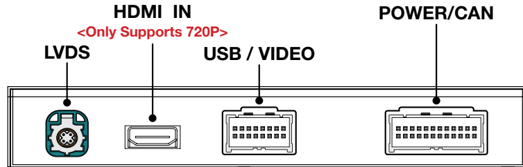
POWER / CAN ADZ-IA67
