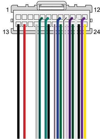
POWER / CAN ADZ-MMI3G
