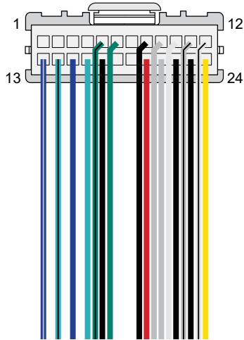
POWER / CAN ADZ-A67
