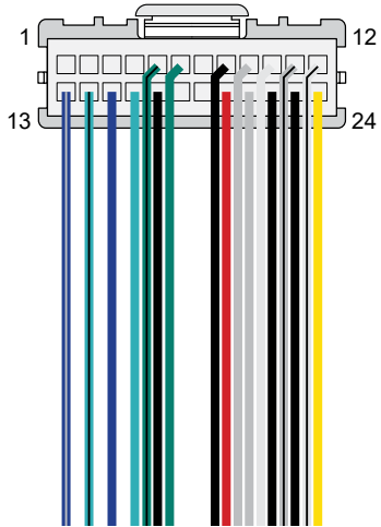
POWER / CAN ADZ-IA67
