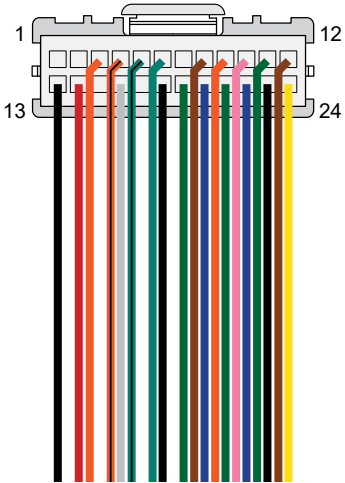
POWER / CAN ADZ-Q3
