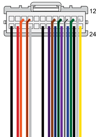
POWER / CAN ADZ-MMI3G
